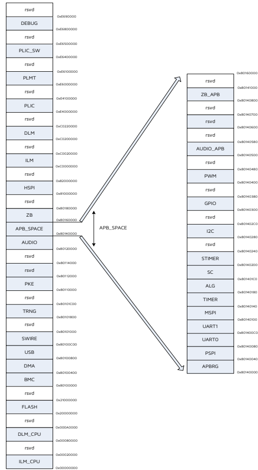
Figure 4-1 Memory Map
