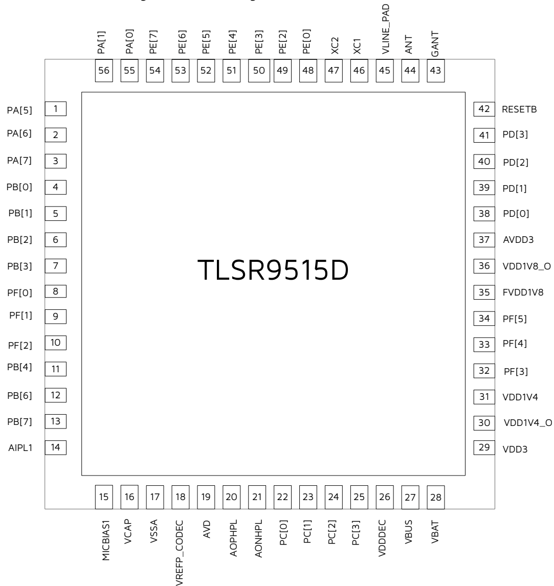
Figure 1-5 Pin Assignment of TLSR9515D
