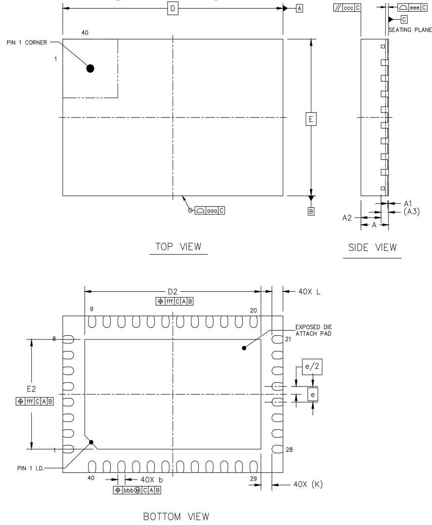
Figure 1-2 Package of TLSR9515A/B
