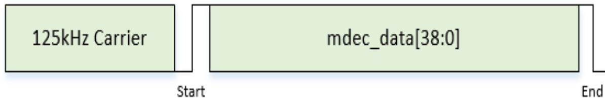
Figure 12-1 Frame Format
