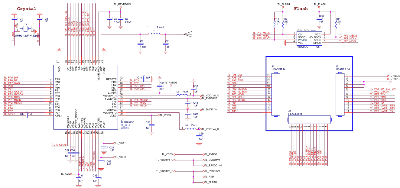
Figure 3-3 Schematic of TLSR9515D
