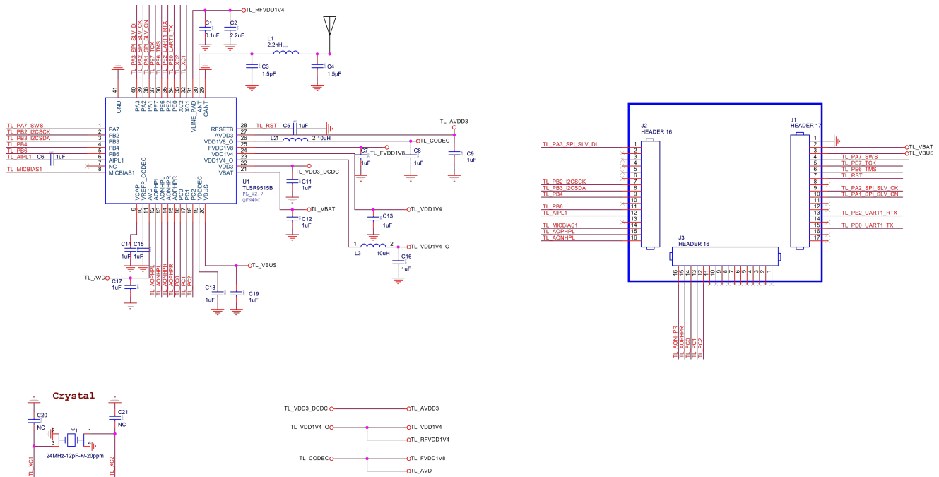
Figure 3-2 Schematic of TLSR9515B
