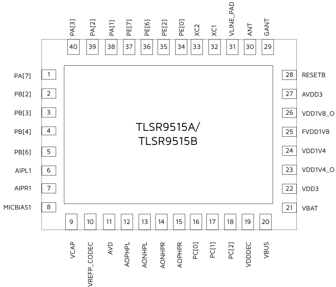
Figure 1-4 Pin Assignment for TLSR9515A/B
