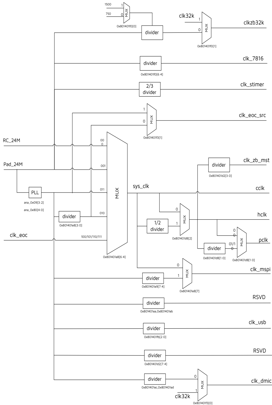
Figure 7-1 Clock Source
