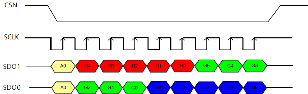
Figure 10-16 RGB666 Pixel Transition
