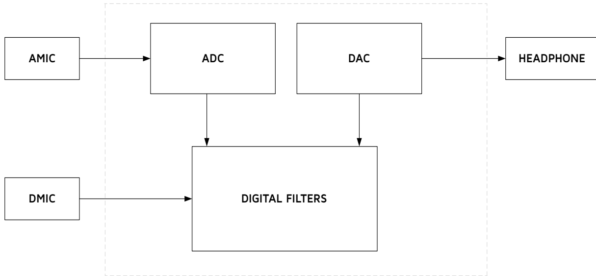
Figure 5-1 Audio CODEC
